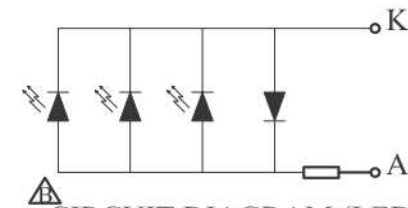
CIRCUIT DIAGRAM (LED1*3 DICES)
