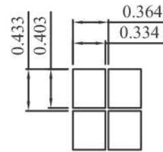
SCALE 20/1
