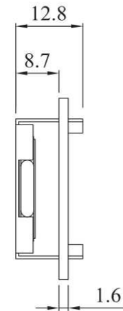
ARRAY LED
