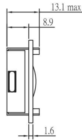
LED B/L
