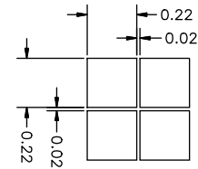
LCD DOTS SCALE:40:1
