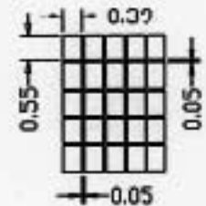
CHARACTER DOT PATTERN
